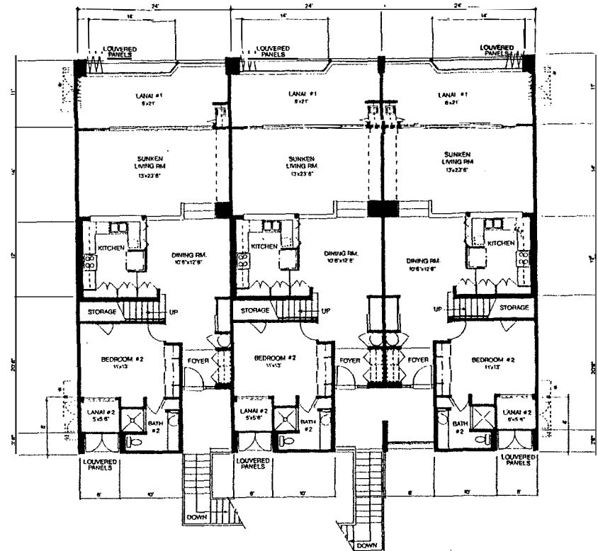
TYPICAL THIRD & MEZZANINE LEVEL
