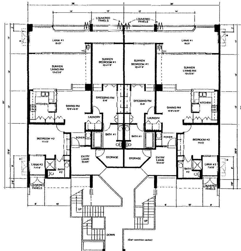
TYPICAL SECOND FLOOR PLANS GROUND FLOOR SIMILAR
